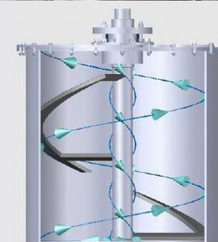
Product Flow
